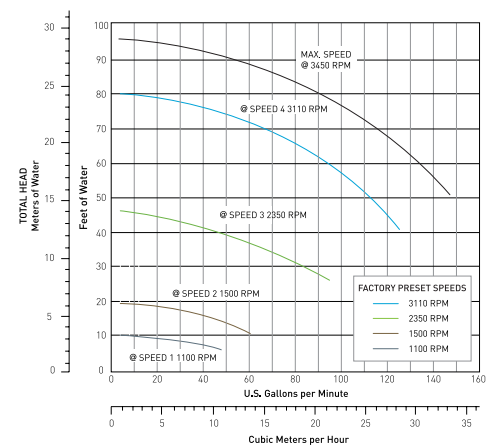
Performance Curves
